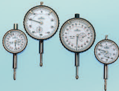
Dial gauges, housing- \varnothing 58 mm and 40 mm
