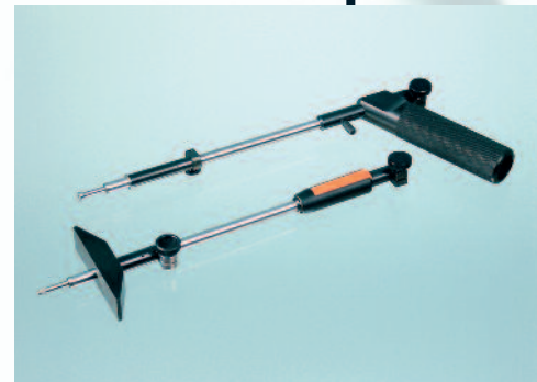
Depth meas. instruments OT - Standard (bottom) and OT 4 (top)
