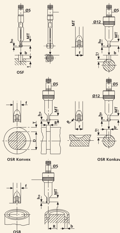
Flachhülsen in Sonderform
